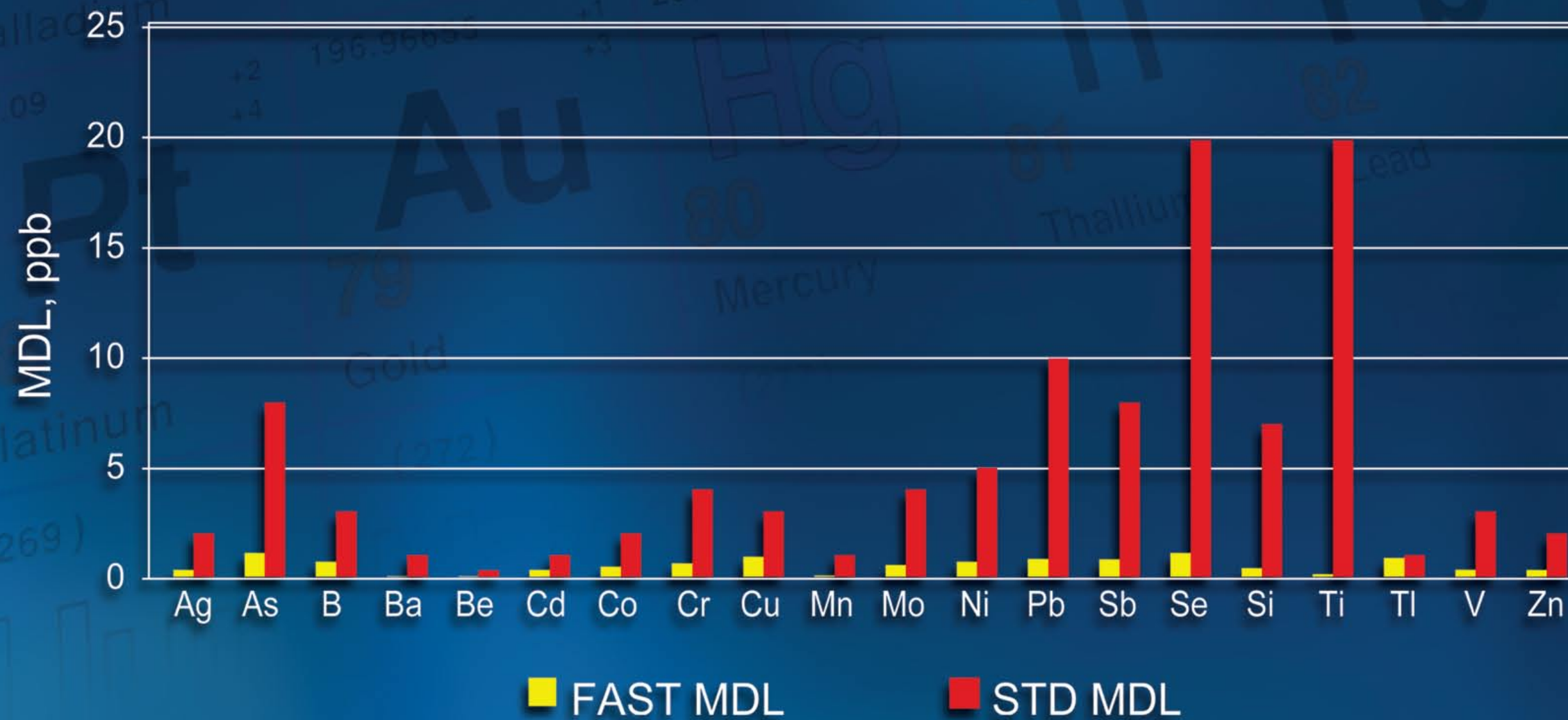
EPA 200.7 MDL Comparison, \mu\text{g/L} (ppb)
